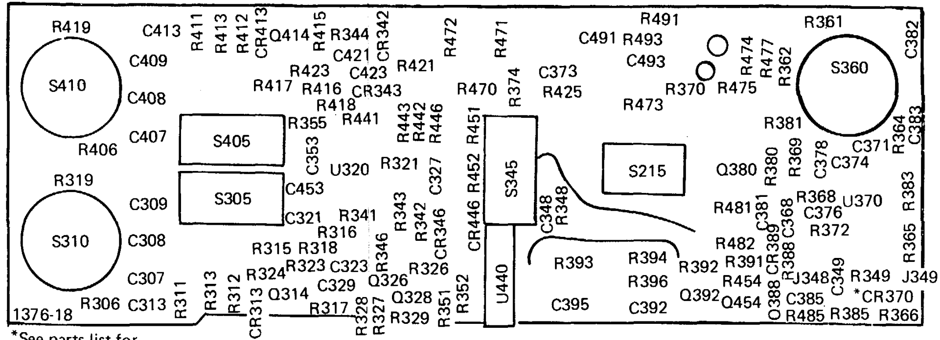
Figure 8-1A. A1 Input Circuit Board (Front).
